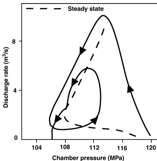
Fig. 11. Evolution of the eruption on a plot of extrusion rate vs. chamber pressure. Arrows show the direction of parameter variation with time. The steady state solution is shown by the dashed line.
